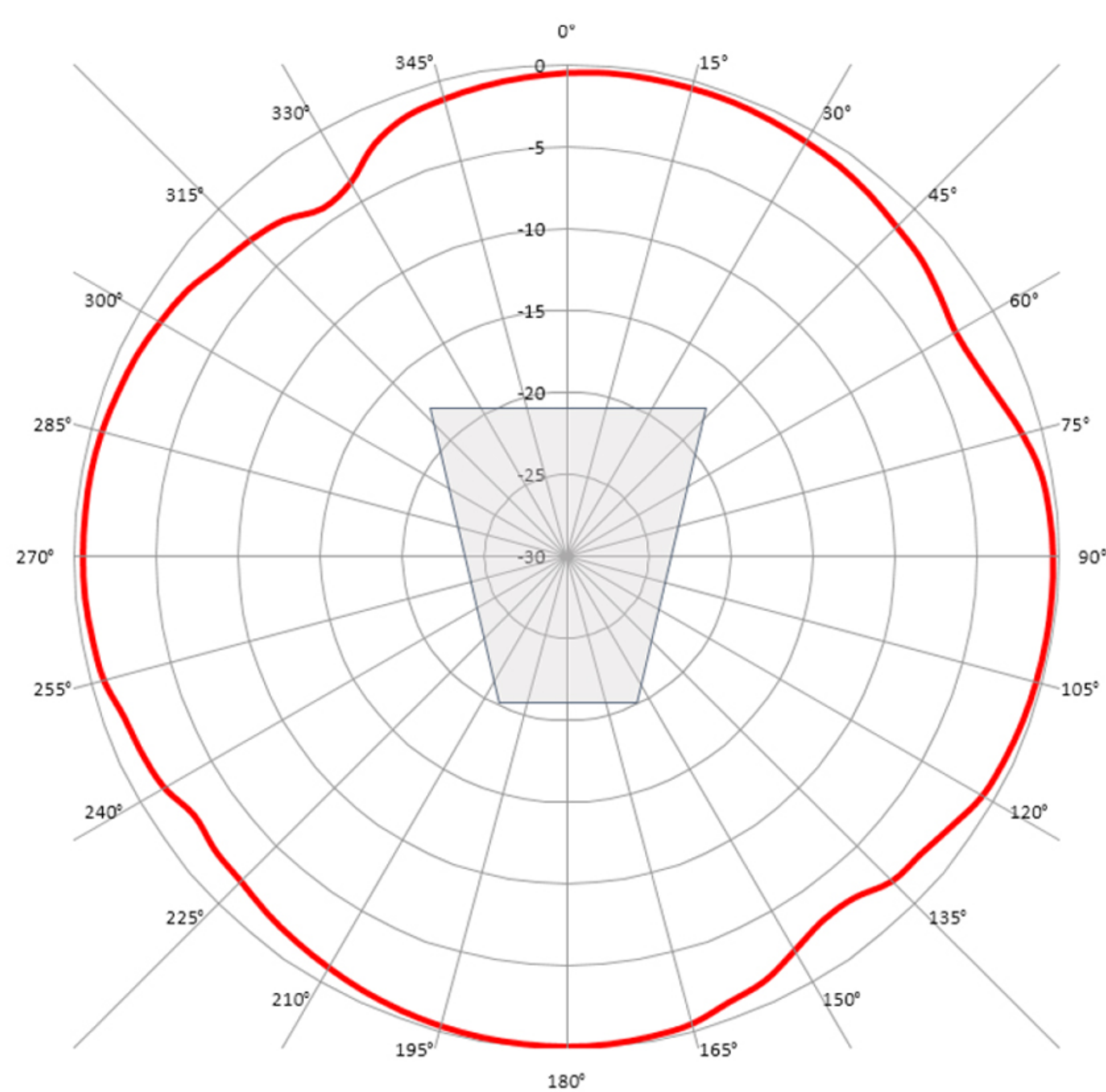
Microphone Array Voice Bandwidth Pickup Polar Pattern
